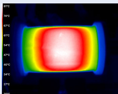
Infra-red photo showing heat concentration at the centre of the mould.
