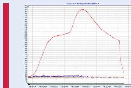
Live Recording of inner mould air temperatures using 493K's K-KORD Software.
